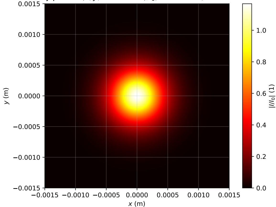
Intensity profile I(x, y, z = 0.796m)/I_0 , P_{in}=0.7P_{cr} , artificial time
